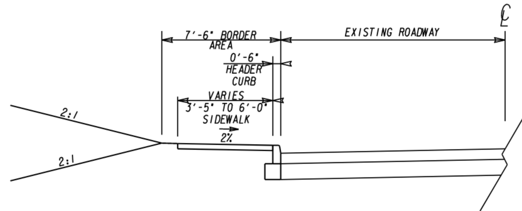
TYPICAL SECTION - NARROW WIDTH CONDITION
