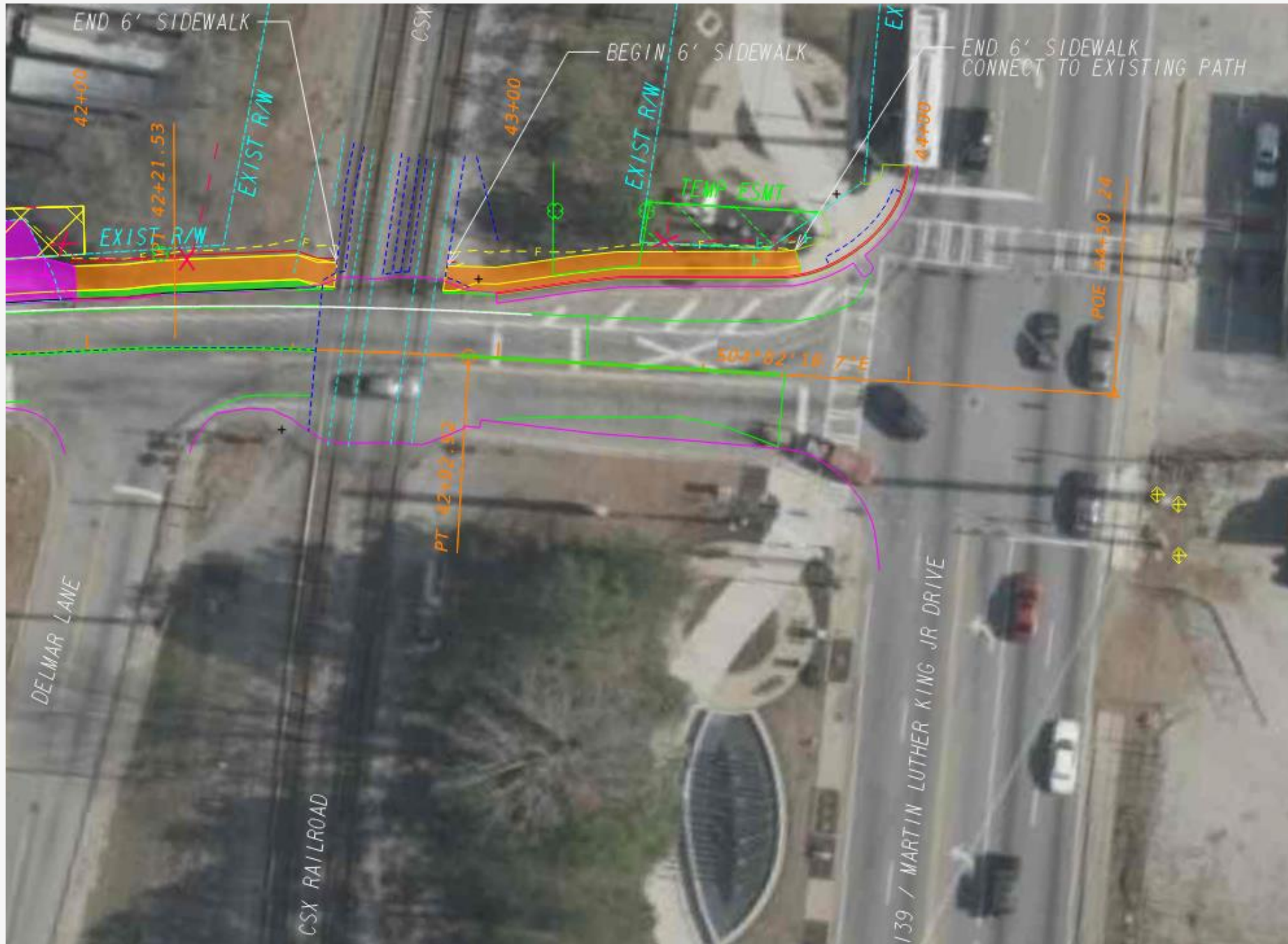
Plan View
