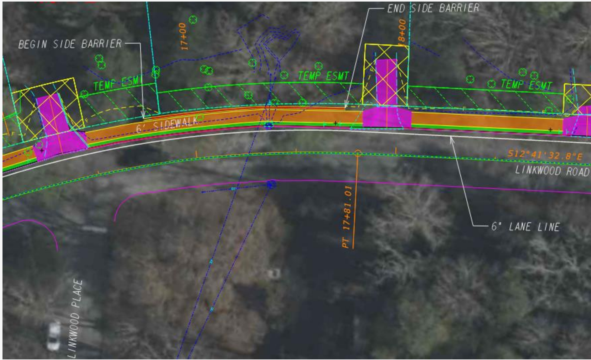
Plan View
